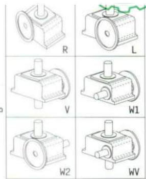
軸向選擇 Shaft Direction
