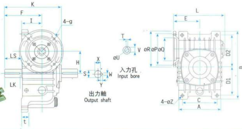
軸向選擇 Shaft Direction
