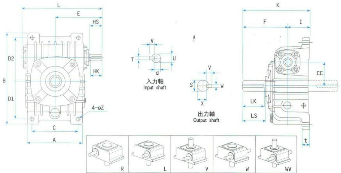
軸向選擇 Shaft Direction
