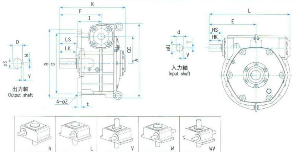
軸向選擇 Shaft Direction
