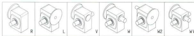
軸向選擇 Shaft Direction
